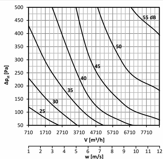
Diagram No. 44 Sound power level L_{WA} [dB(A)] radiated outside the pipeline DN500, with insulation
