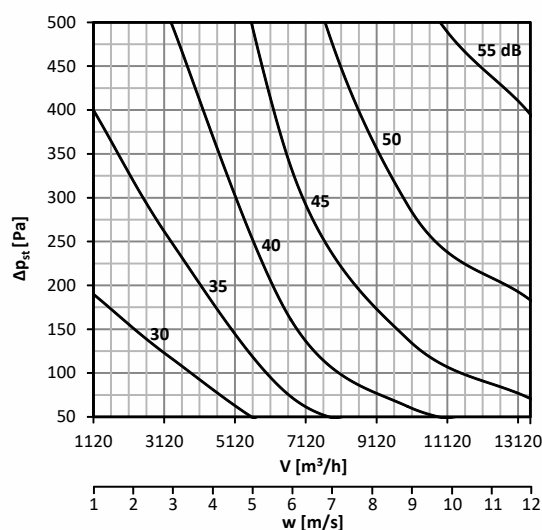
Diagram No. 45 Sound power level L_{WA} [dB(A)] radiated outside the pipeline DN630, with insulation
