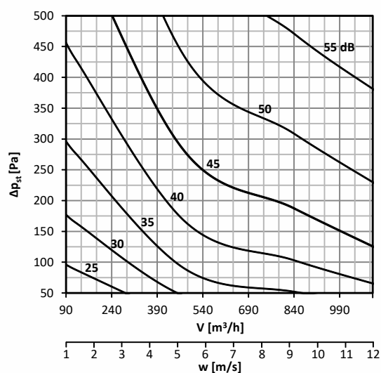
Diagram No. 21 Sound power level L_{WA} [dB(A)] radiated outside the pipeline DN180, without insulation
