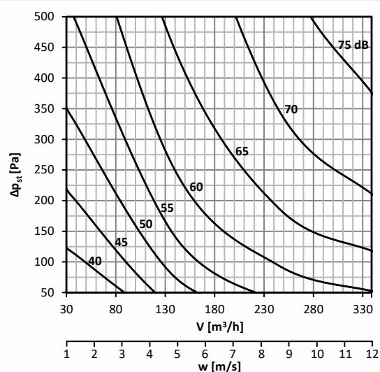
Diagram No. 4 Sound power level L_{WA} [dB(A)] inside the pipeline DN140
