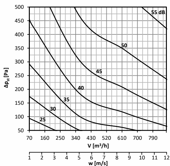
Diagram No. 20 Sound power level L_{WA} [dB(A)] radiated outside the pipeline DN160, without insulation
