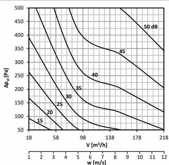
Diagram No. 18 Sound power level L_{WA} [dB(A)] radiated outside the pipeline DN125, without insulation
